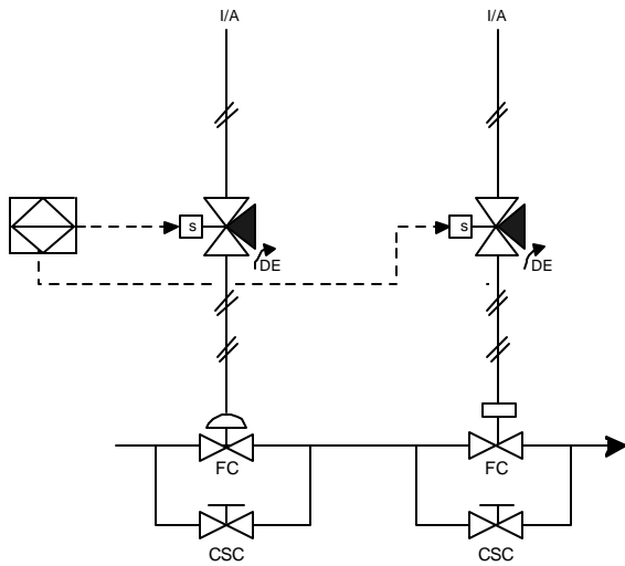
Figure 2.6.E: Installation Illustration for Final elements Showing 1oo2 Valves and 1oo2
