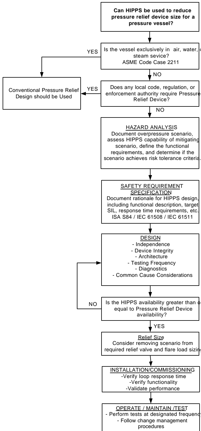
Figure 2.6.A: Simplified Design Tree
